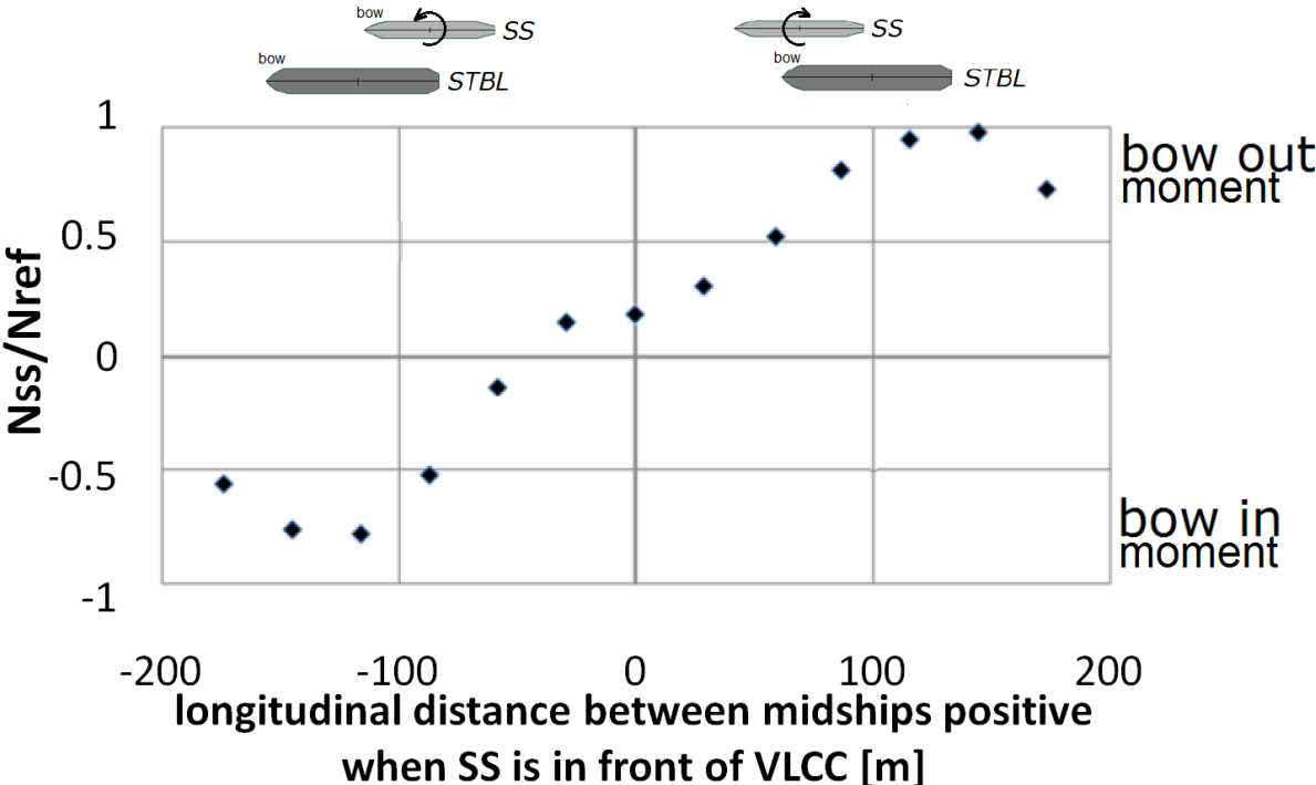
Figure 1 Yaw moment of SS at one lateral distance and different longitudinal distances to the STBL
